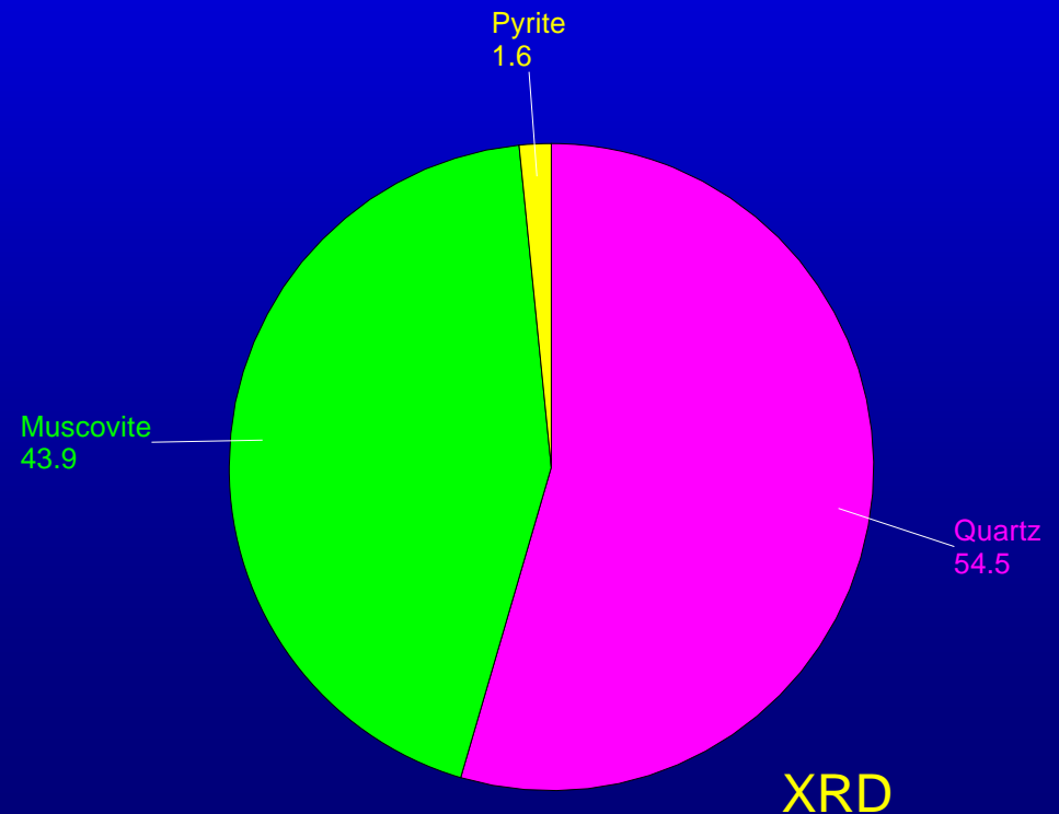
Volcanic Dacite - Rietveld XRD
