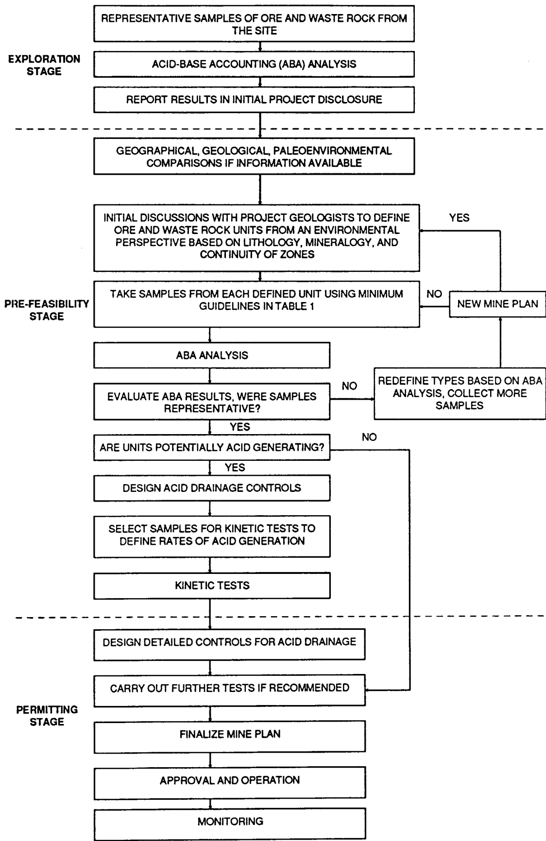
Figure 1. Procedure for Evaluating the Potential for Acid Generation at a Mine Site
